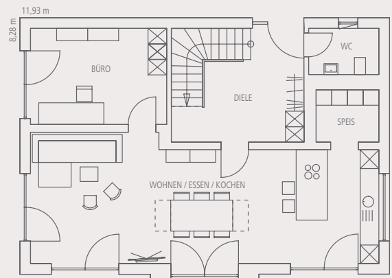
EG, 81 m 2 WF
